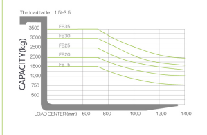
CAPACITY CHART
