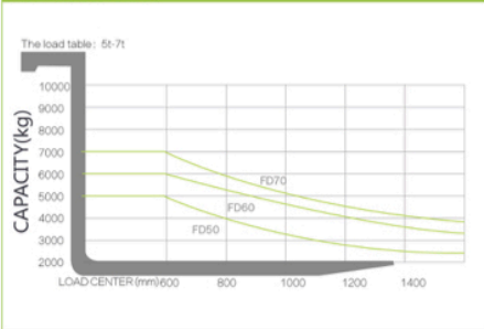
CAPACITY CHART
